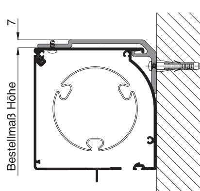
Wandmontage
