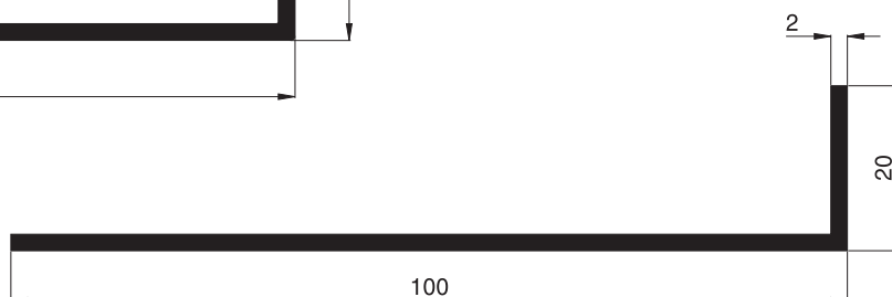
10 91 40 Winkelprofil 100/20/2
