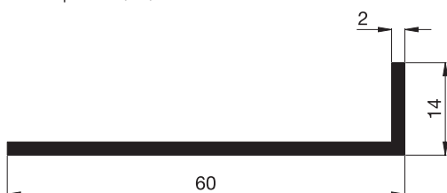
10 91 08 Winkelprofil 60/14/2
