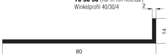
10 91 28 Winkelprofil 80/14/2
