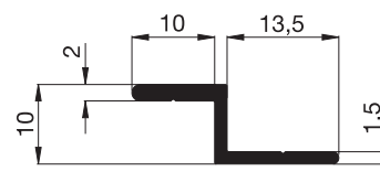
10 28 10 Z-Winkelprofil
